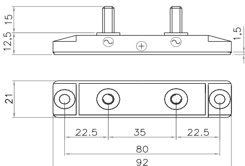
Fig.10 MK400.02NI-MM6x15-FIX5-LP-P80-TA
